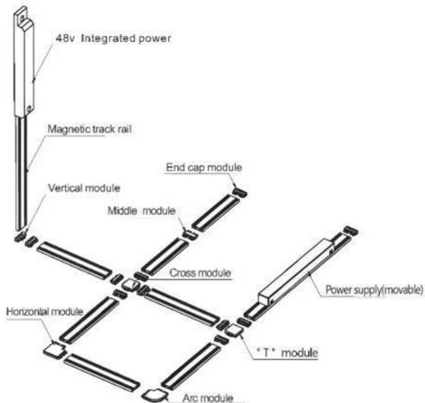
Schematic diagram of magnetic light track connection
